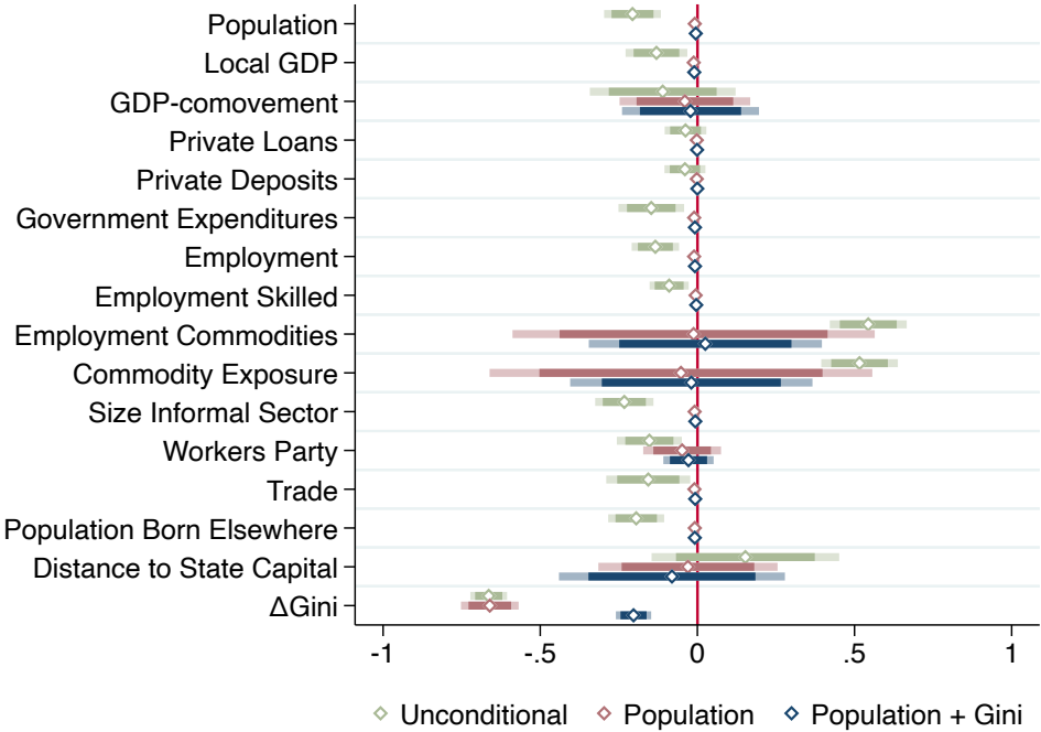
Figure 2: Covariate Balance
